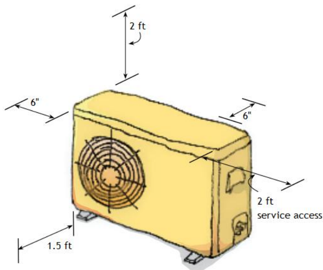
Figure 28. Outdoor Split Unit Clearances
